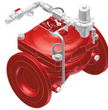
Figure 2. Deluge Valve
