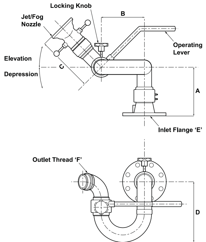
Figure 1. Fixed Deck Monitor
