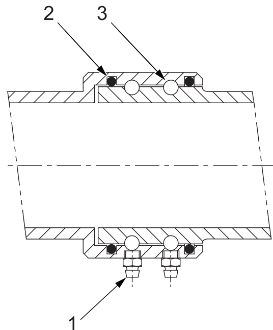
Figure 2. Section showing details of bearings
